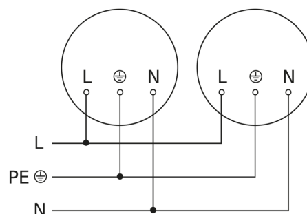
Circuit diagram
